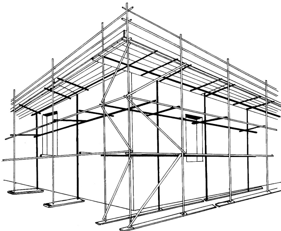
Figure Tube-and-coupler scaffold
