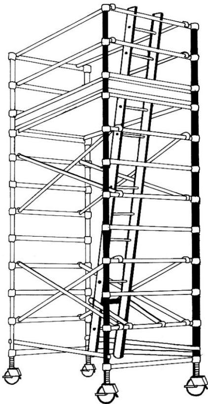
Figure Prefabricated scaffold (tower frame type)
