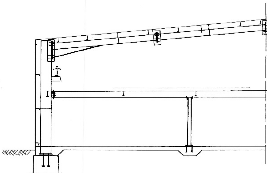
Figure Steel erection
