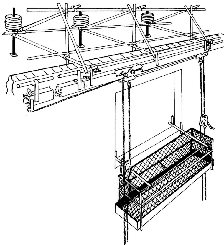
Figure 2 Suspended scaffold (swing stage type)
