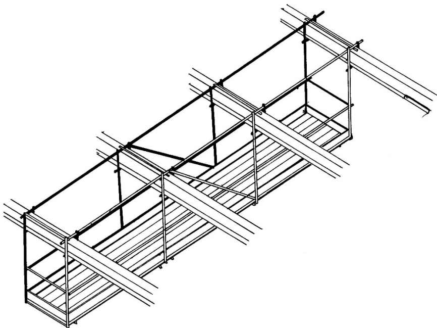
Figure 1 Hung scaffold
