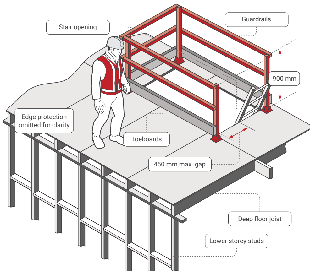
Figure 21 Void at upper level guarded
