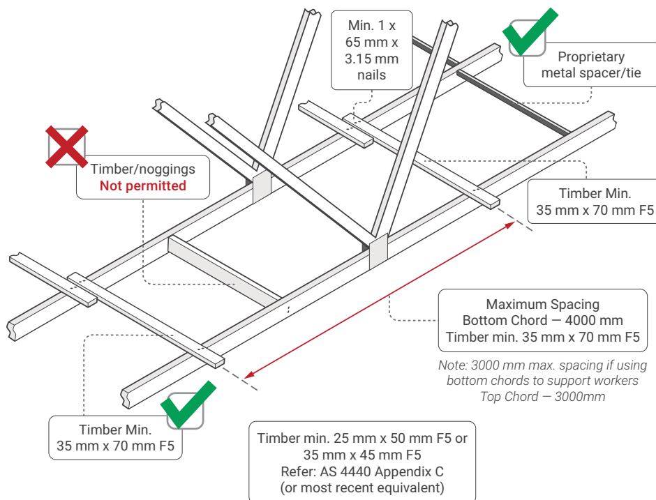
Figure 28 Temporary bracing ties to bottom chord of trusses. Note: Bracing to top chord similar
