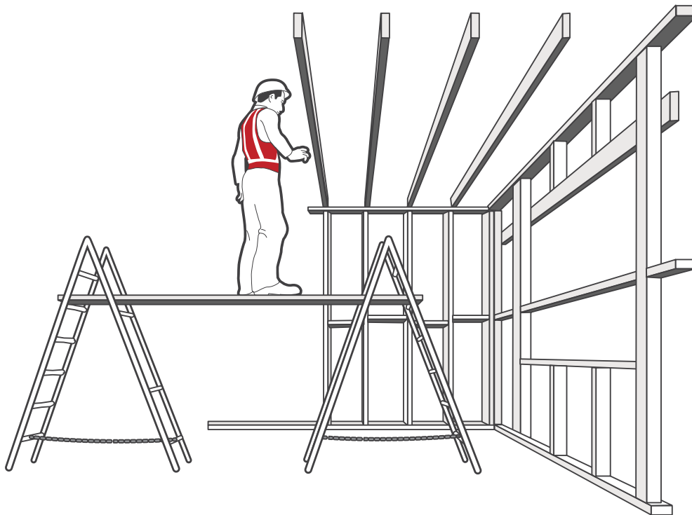
Figure 20 Installing ceiling or upper level floor joists
