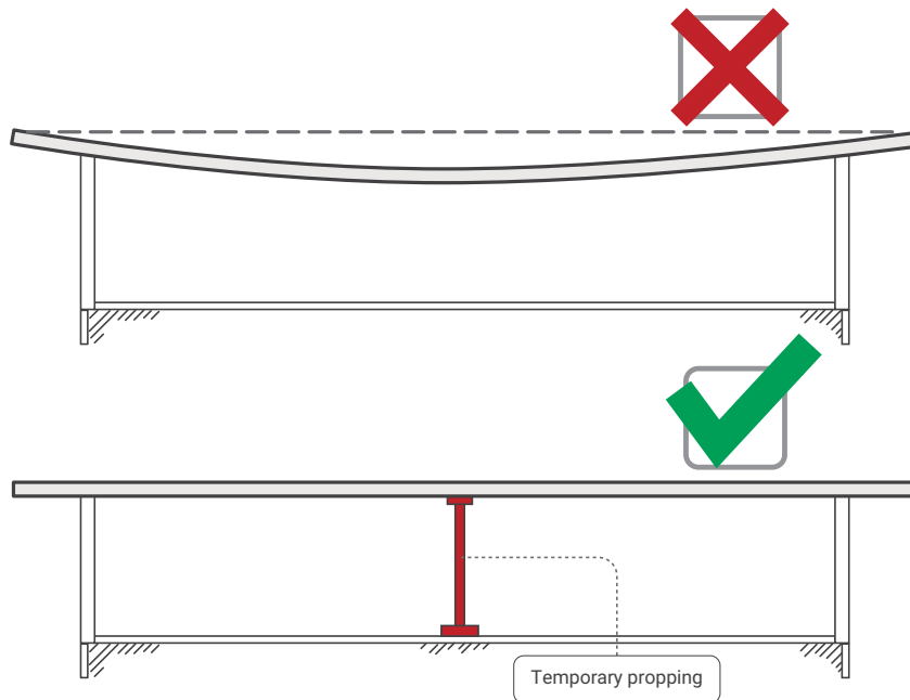
Figure 23 Method of supporting long trusses
