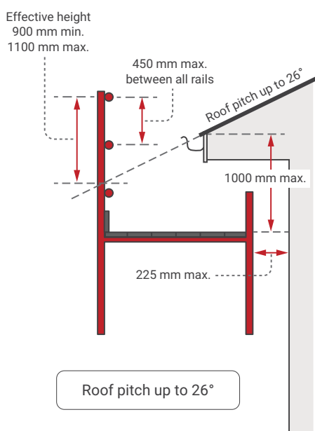
Figure 30 Catch platforms for roofing work
