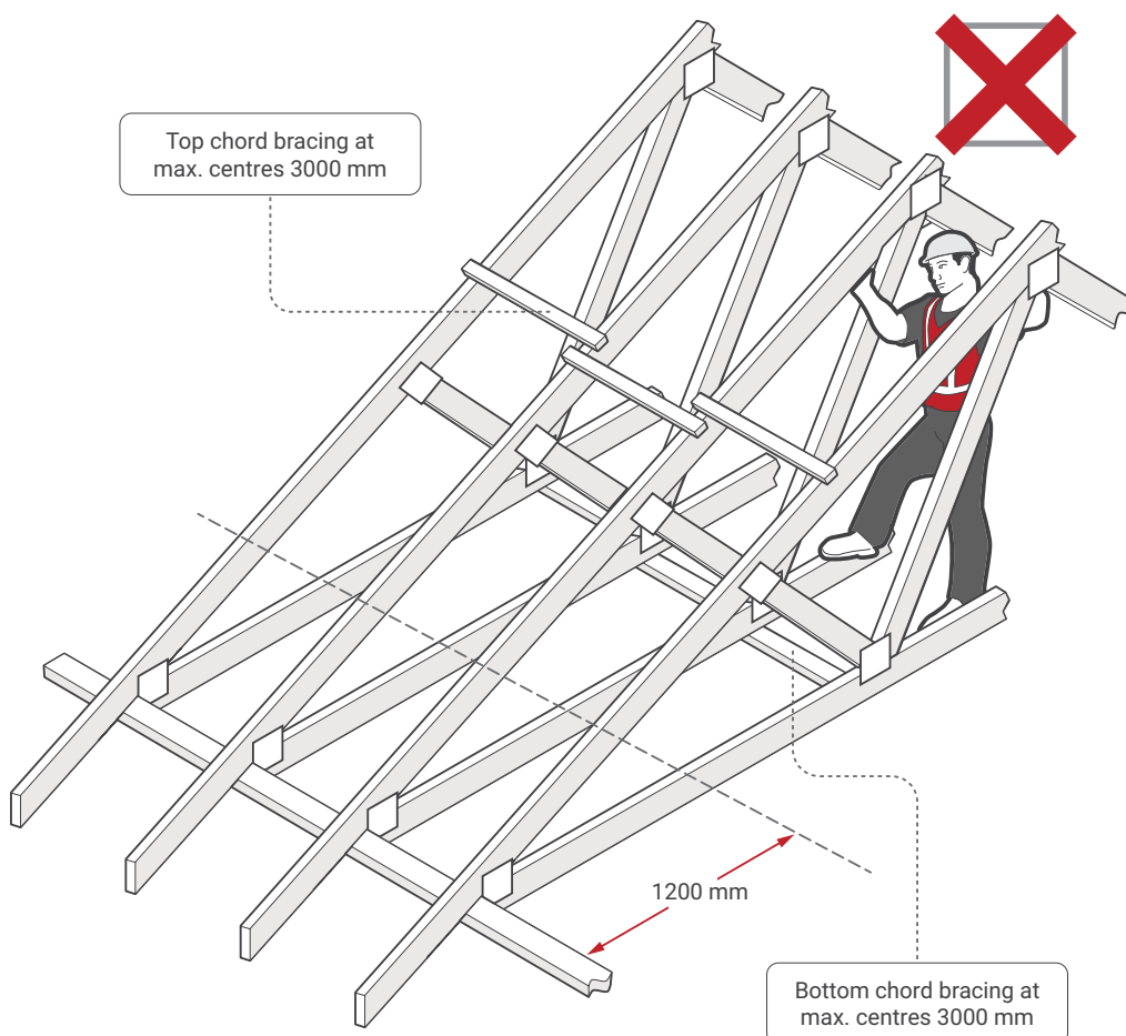
Figure 24 No go zone for persons erecting trusses
