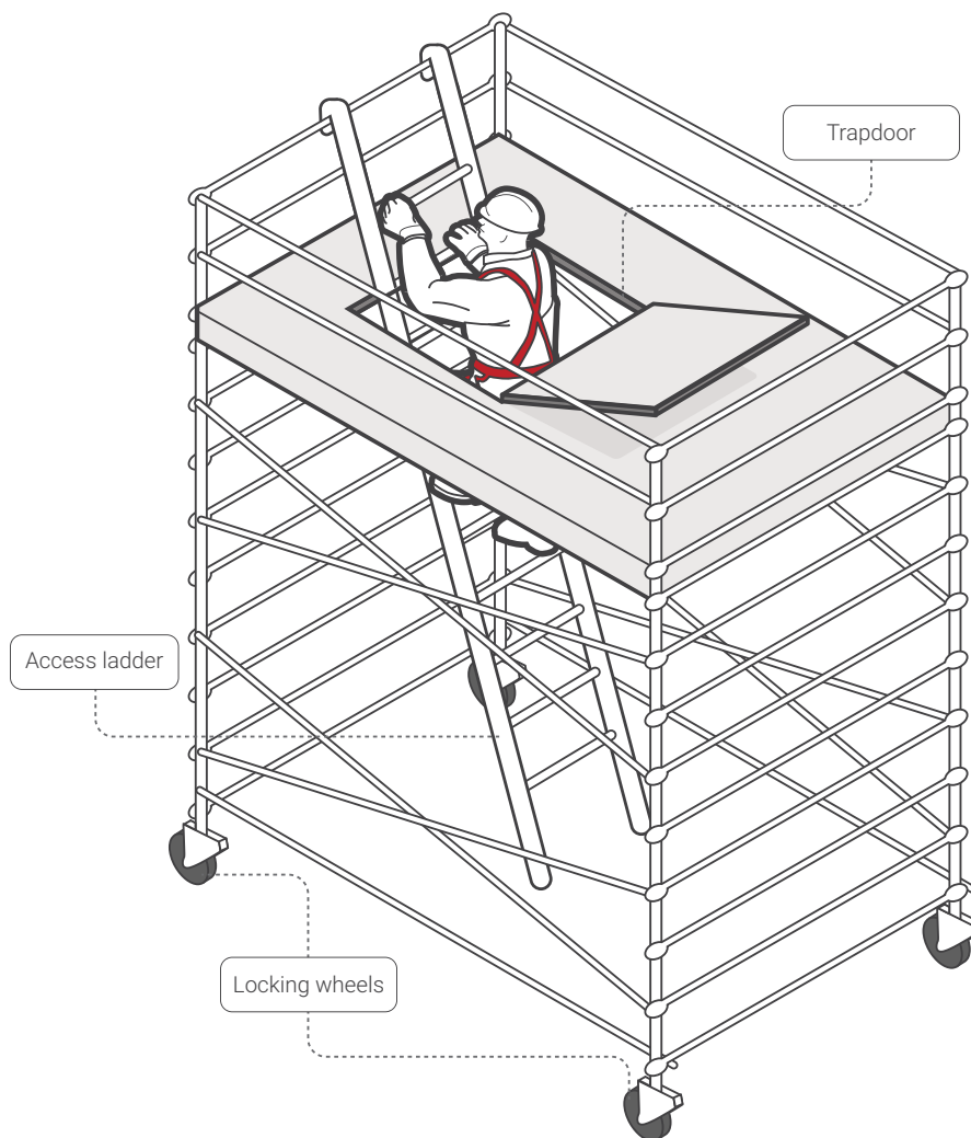
Figure 4 Mobile scaffold with access ladder
