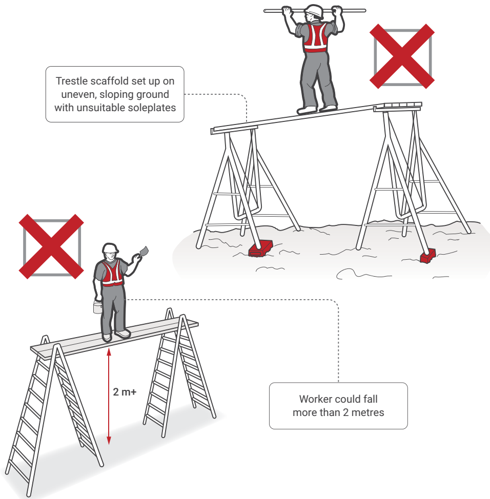
Figure 6 Examples of incorrectly used trestle scaffolds
