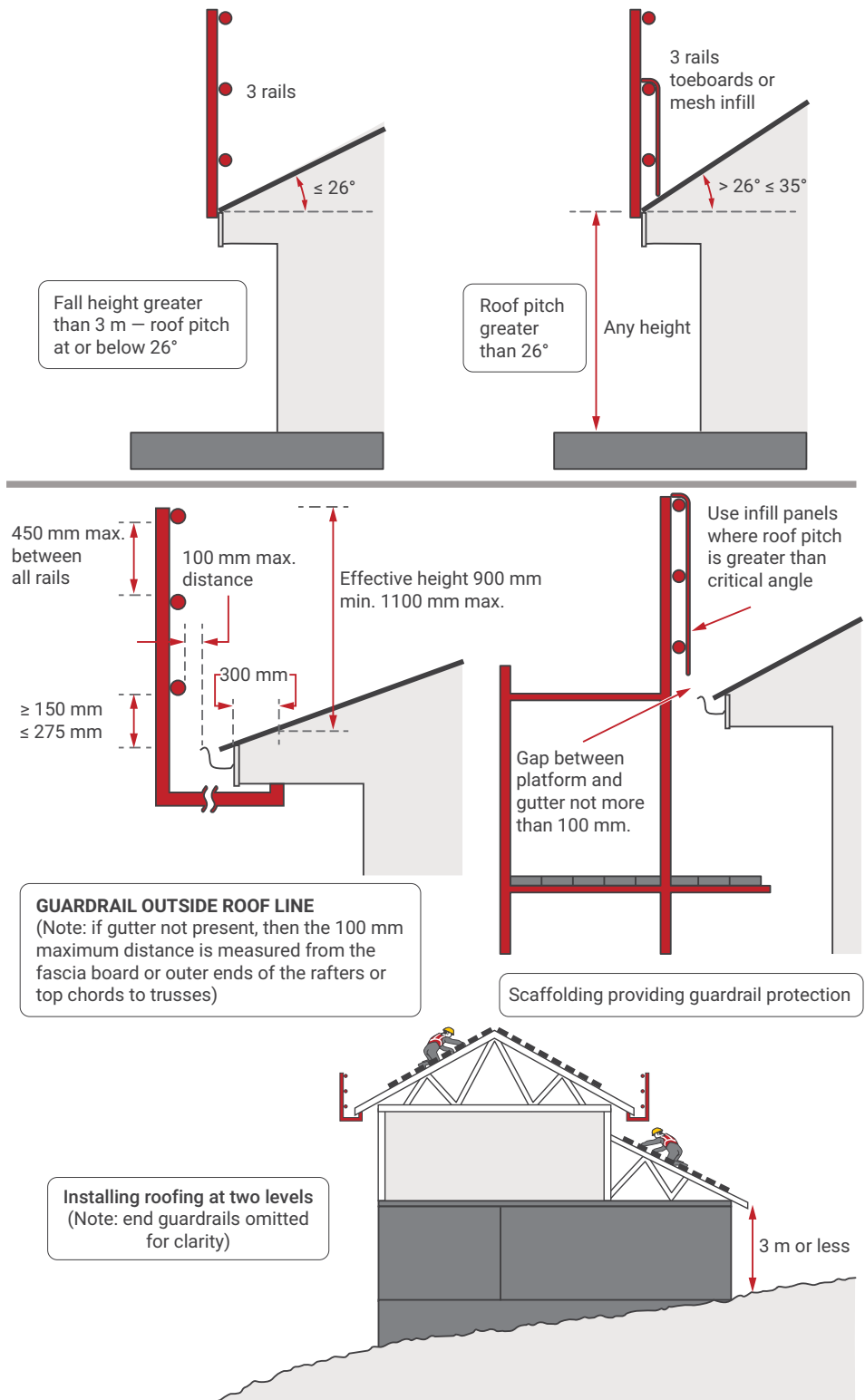
Figure 32 Guardrail systems for roofing work
