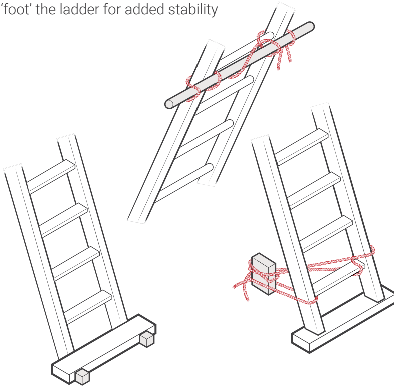
Figure 14 Examples of effectively securing a ladder
