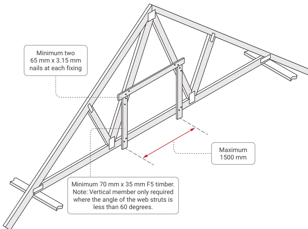
Figure 25 Suggested method of fixing temporary waling plate
