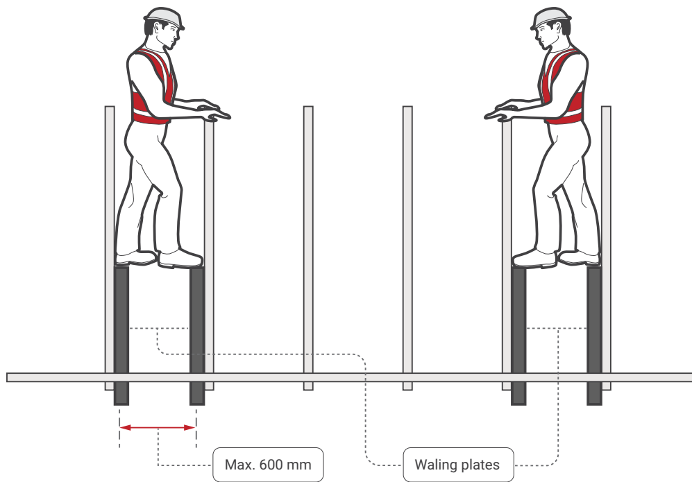
Figure 26 Showing the positions for pairs of waling plates
