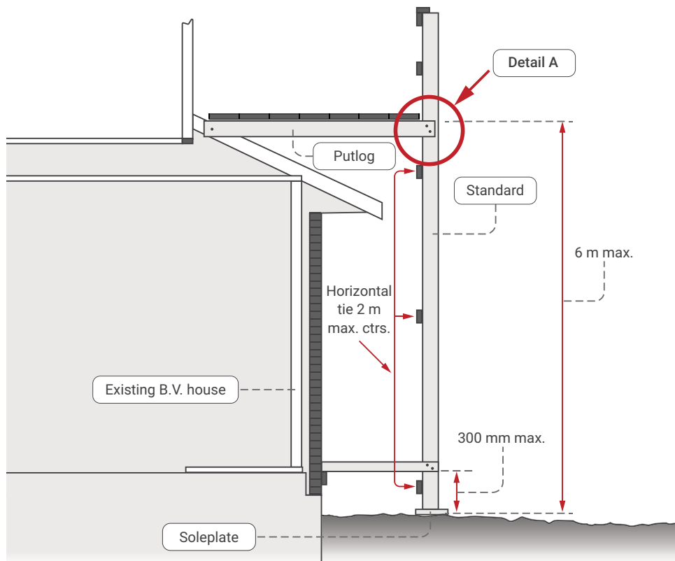
Figure 34 Timber scaffold (single pole – high first lift)
