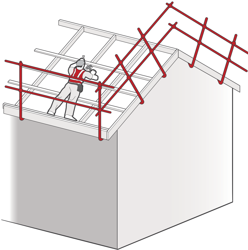
Figure 31 Fixing roof battens to trusses
