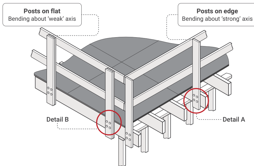
Figure 9 Timber guard rails – posts subject to bending about their weak and strong axes
