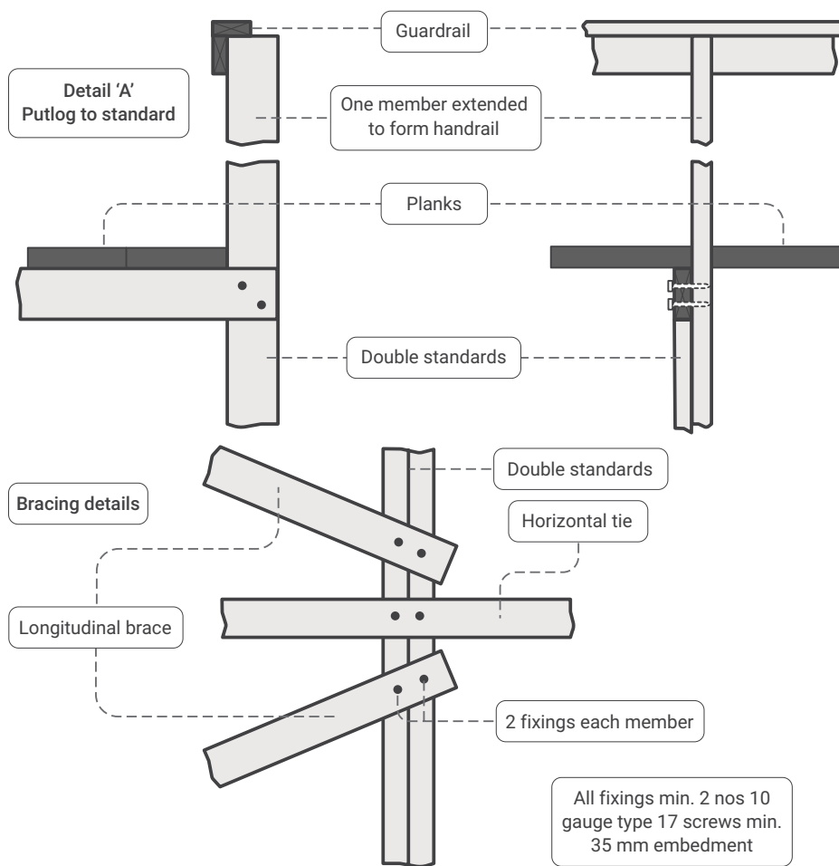
Figure 35 Timber scaffold (single pole – high first lift) details
