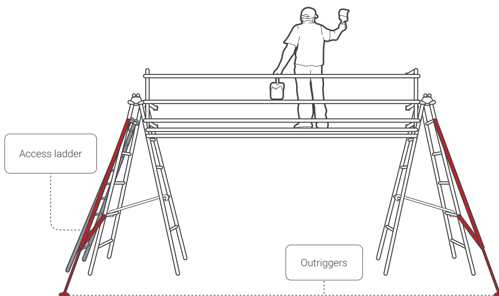
Figure 5 Trestle ladder scaffold with guardrailing and outriggers for stability
