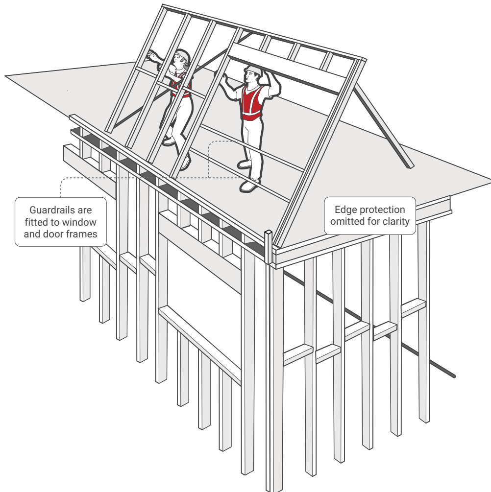
Figure 22 Erecting upper level wall frames
