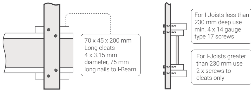
Detail 'A' Bending about strong axis: I-Beam joists
