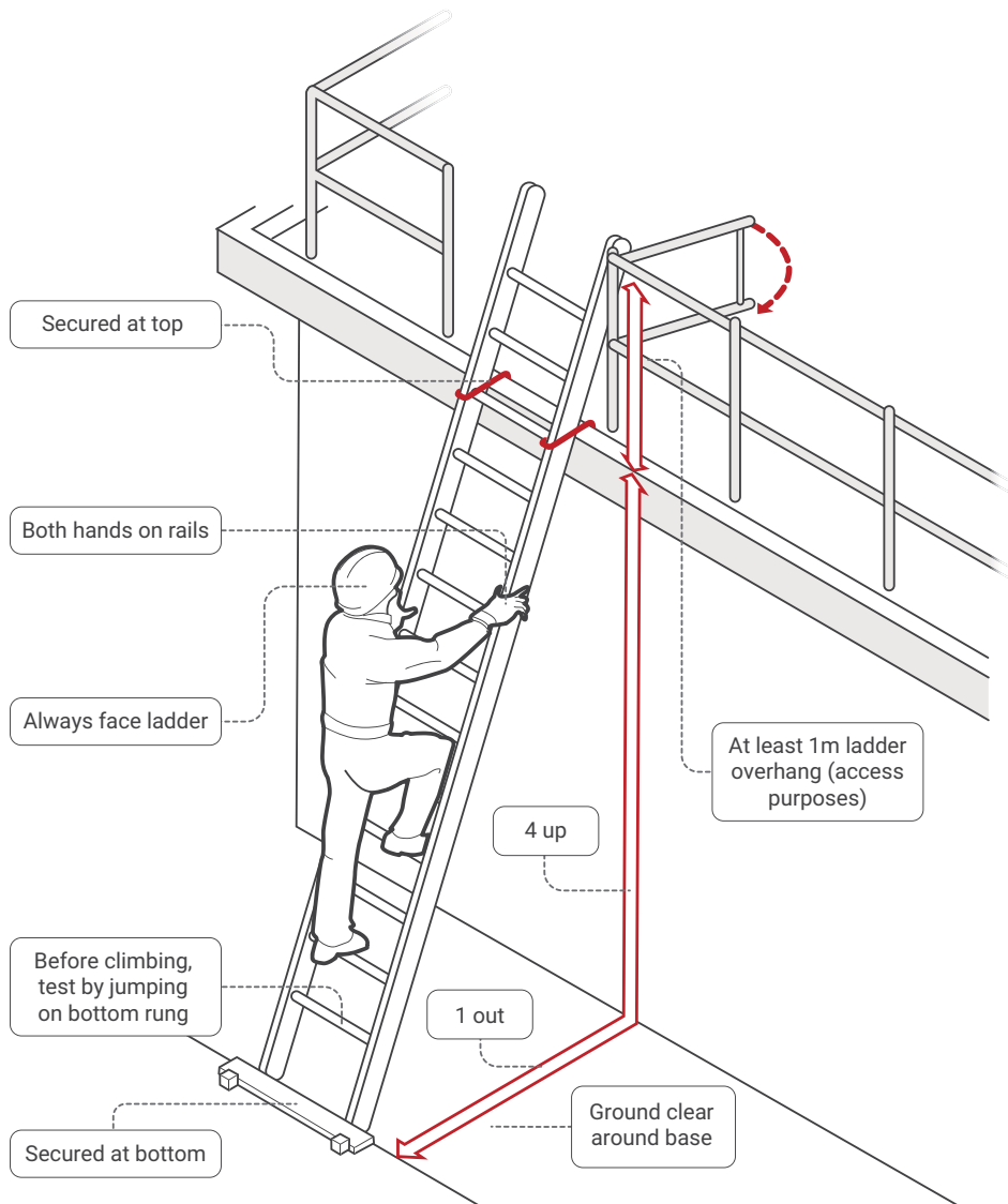
Figure 15 Example of acceptable ladder use
