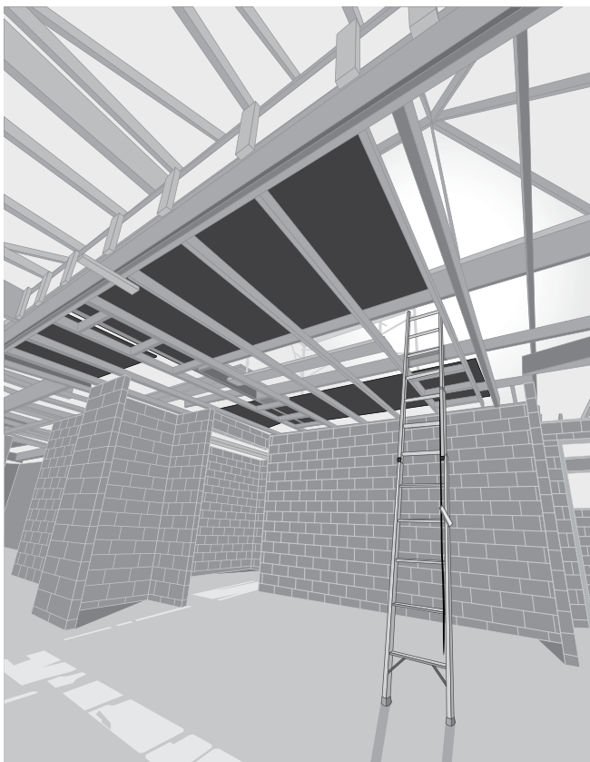
Figure 29 A temporary work platform (working deck) in use
