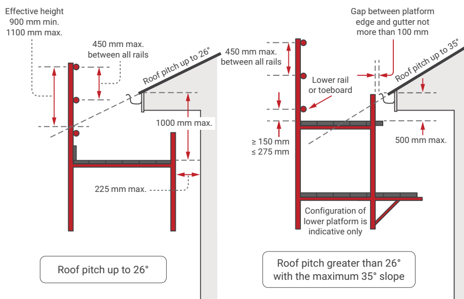
Figure 33 Catch platforms for roofing work
