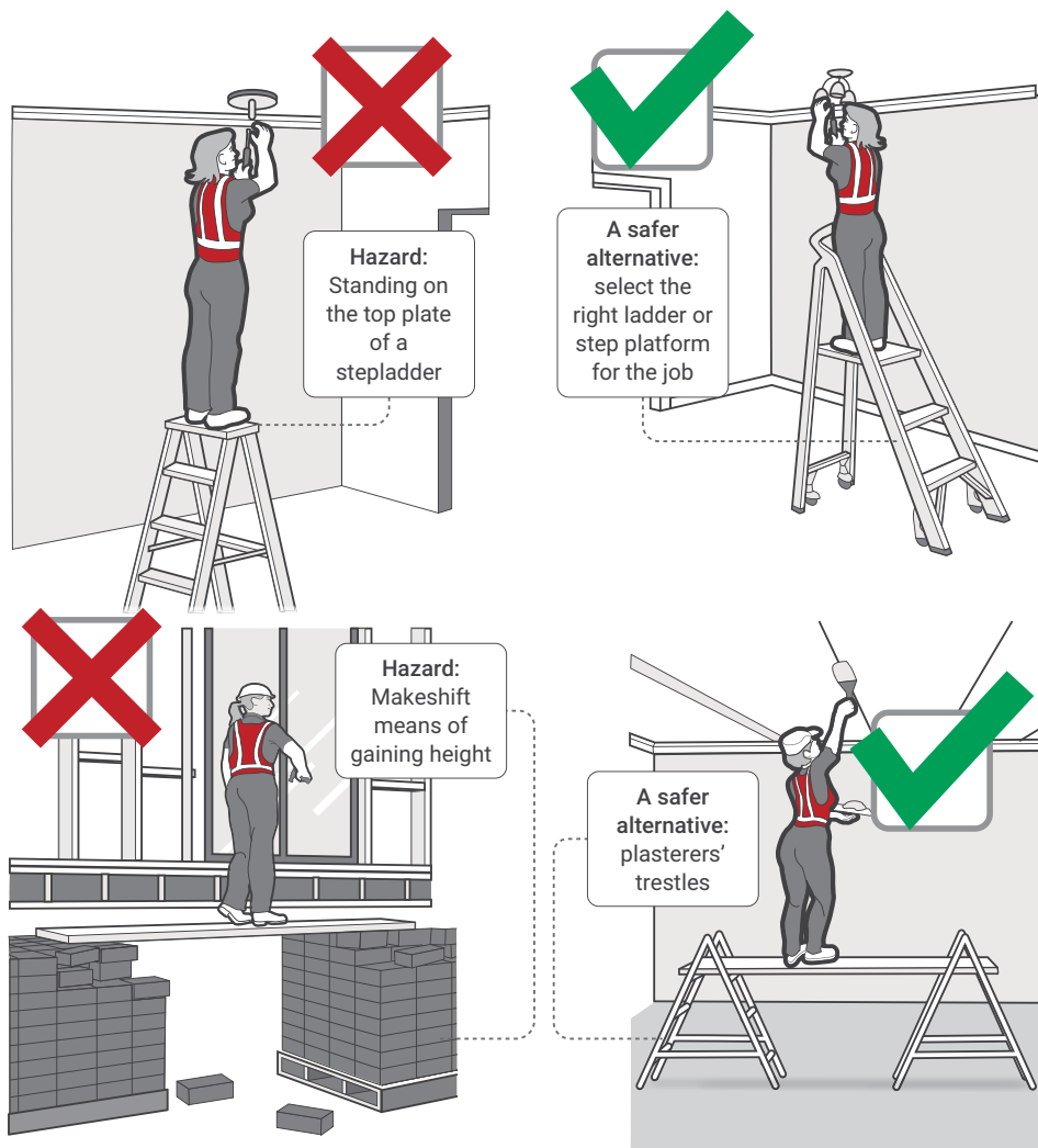
Figure 13 Common work tasks performed at low heights
