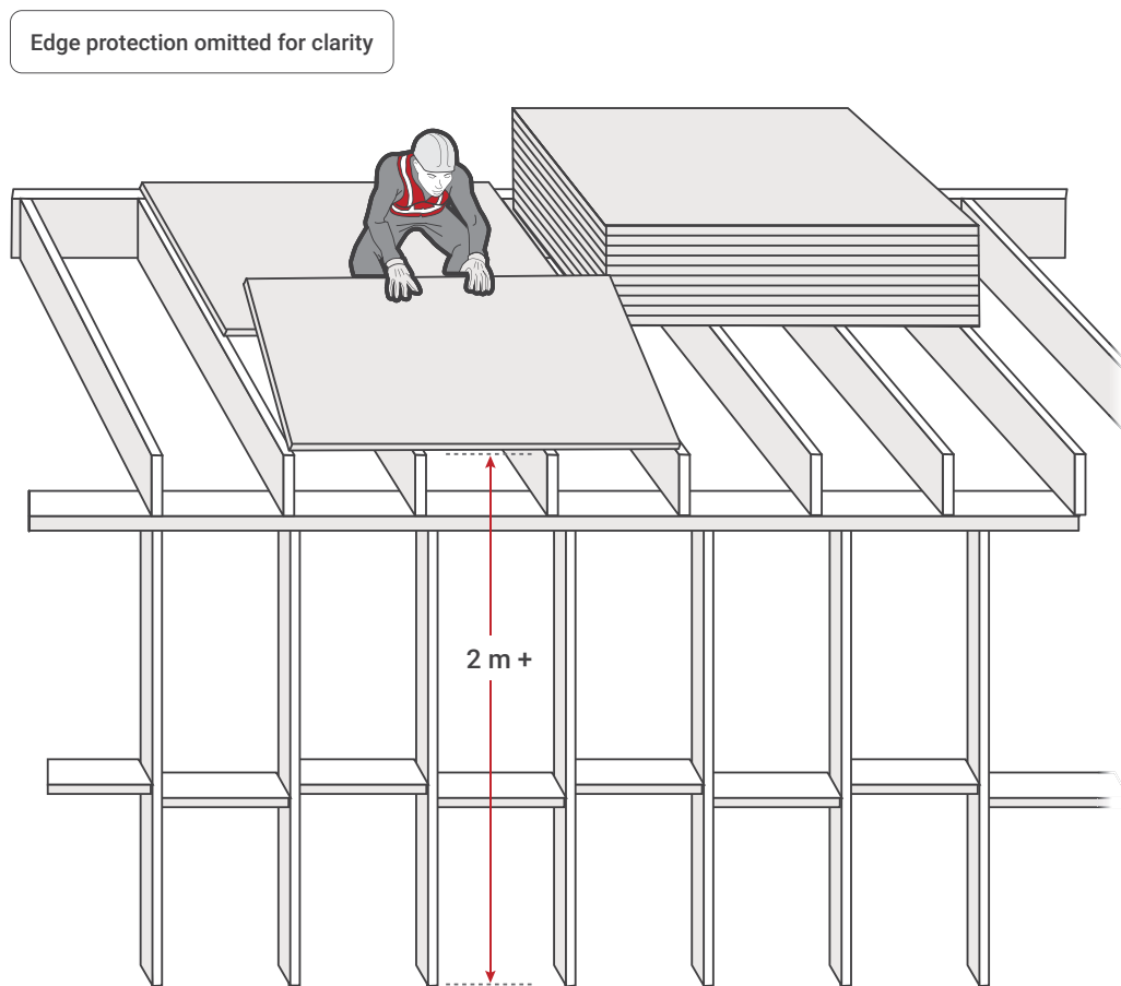
Figure 17 Laying sheet flooring at upper level
