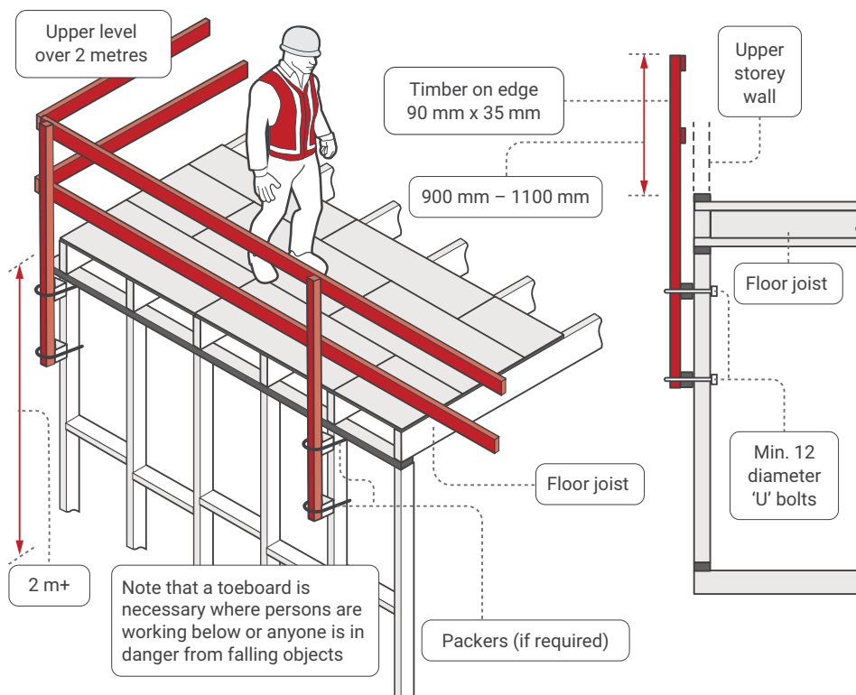
Figure 19 Examples of upper floor edge protection (timber guardrailing)
