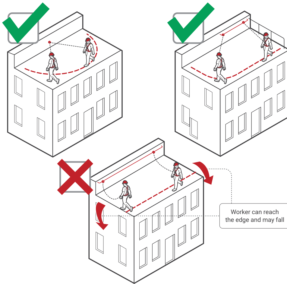
Figure 11 Restraint technique options
