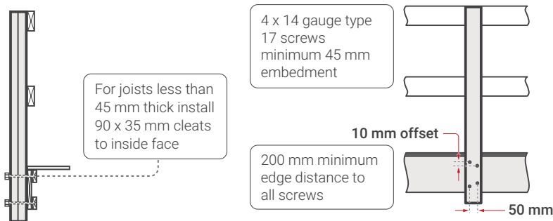
Detail 'B' Bending about weak axis
