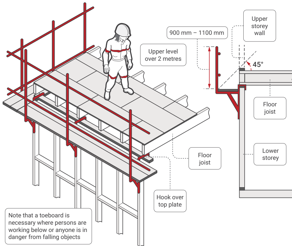
Figure 18 Examples of upper floor edge protection (external scaffolding)
